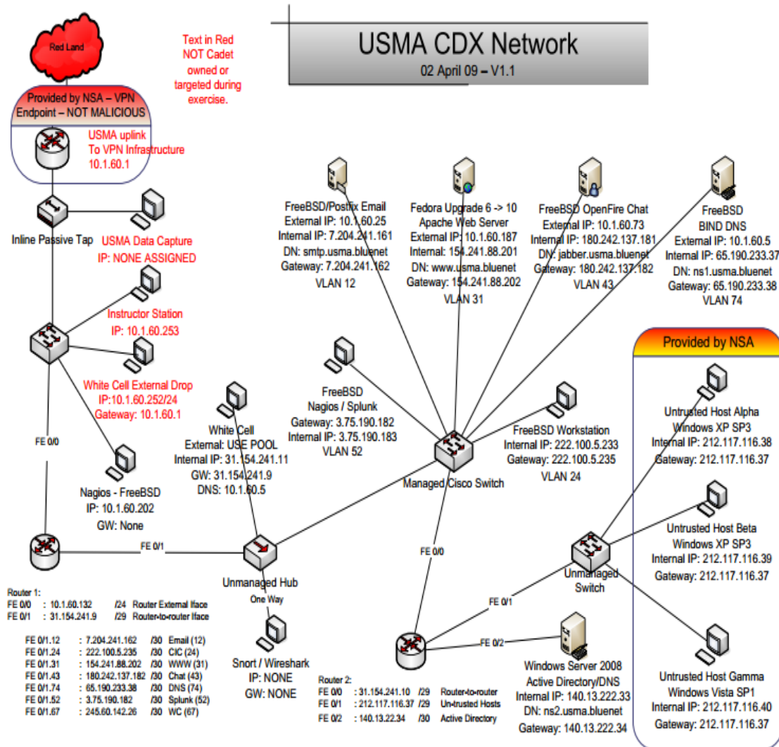
Diagram 3 USMA CDX Network Layout used in a CDX Cyber Range
